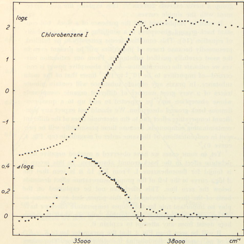
Fig. 16. \log \epsilon (25° C) and \Delta \log \epsilon for chlorobenzene.
