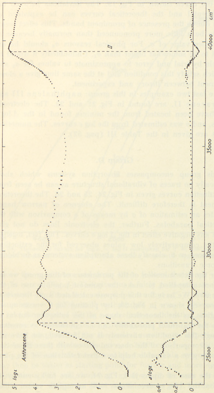
Fig. 22. \log \epsilon (25° C) and \Delta \log \epsilon for anthracene.
