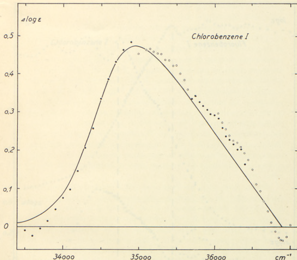
Fig. 14. \Delta \log \epsilon for chlorobenzene I. The different signatures for the observed points indicate four different series of measurements. The theoretical curve is calculated from (16) for \log(c_a K_a / c_b K_b) = 4.7 .
