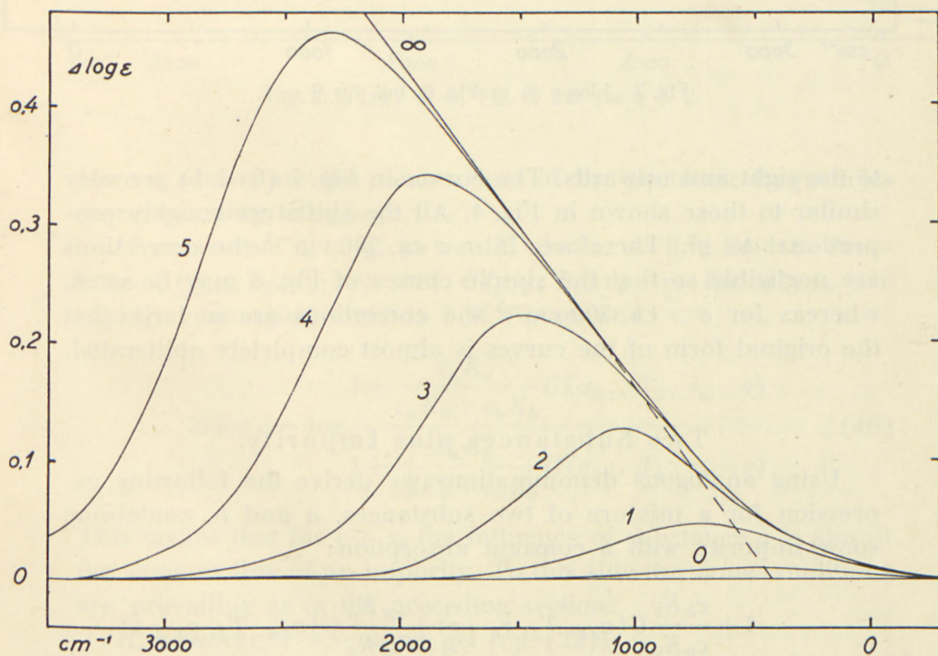
Fig. 6. \Delta \log \epsilon calculated from (38) for \sigma_1 = 300 \text{ cm}^{-1} , \theta = 0 , T_1 = 298^\circ \text{K} and T_2 = 343^\circ \text{K} . The numbers at the curves represent the parameter \log(cK/c_0K_0) . The dotted line is the asymptote calculated from (32).
