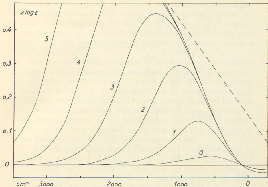
Fig. 8. \Delta \log \epsilon as in Fig. 6, but for \theta = 2 .
