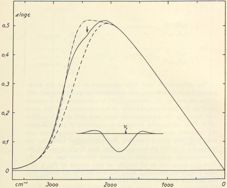
Fig. 10. The effect of a single, prominent band on \Delta \log \epsilon : ---- calculated from (16), — from (59) for \nu_a - \nu_1 = 2400 \text{ cm}^{-1} , and -·-·- from (16), but corrected for the presence of the narrow band. Inserted; the difference between ---- and —.
