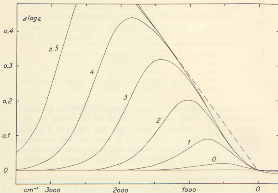
Fig. 7. \Delta \log \epsilon as in Fig. 6, but for \theta = 1 .
