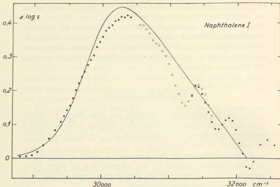
Fig. 11. \Delta \log \epsilon for naphthalene I. The different signatures for the observed points indicate three different series of measurements. The theoretical curve is calculated from (16) for \log(c_a K_a / c_b K_b) = 4.5 .
