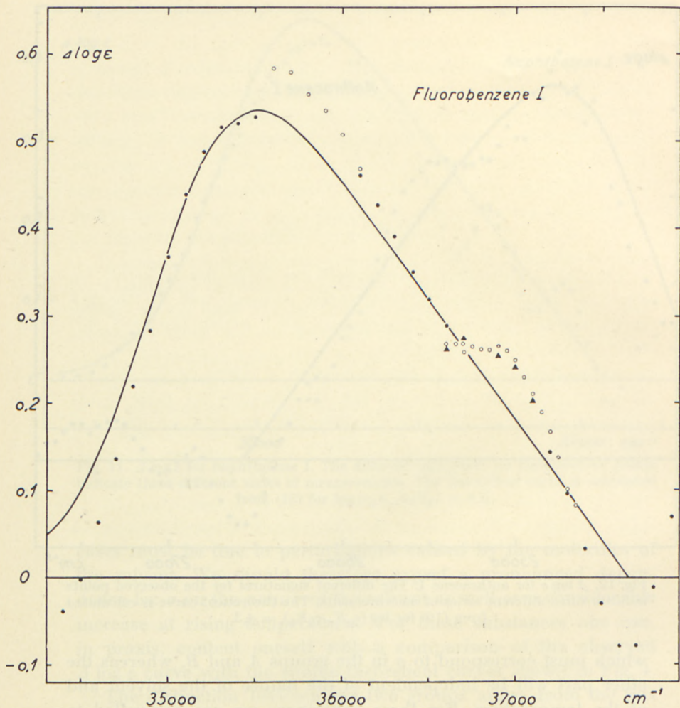
Fig. 13. \Delta \log \epsilon for fluorobenzene I. The different signatures for the observed points indicate six different series of measurements. The theoretical curve is calculated from (16) for \log(c_a K_a / c_b K_b) = 5.2 .
