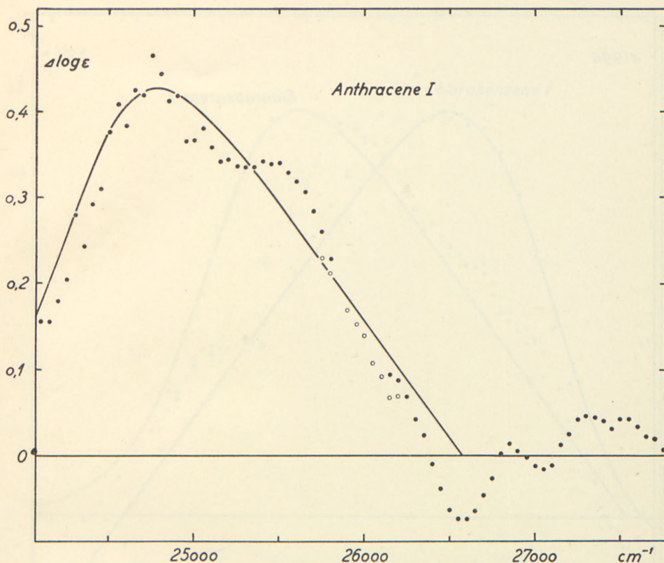
Fig. 12. \Delta \log \epsilon for anthracene I. The different signatures for the observed points indicate three different series of measurements. The theoretical curve is calculated from (16) for \log(c_a K_a / c_b K_b) = 4.3 .
