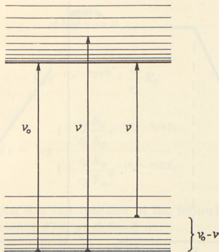
Fig. 1. Energy level diagram.
