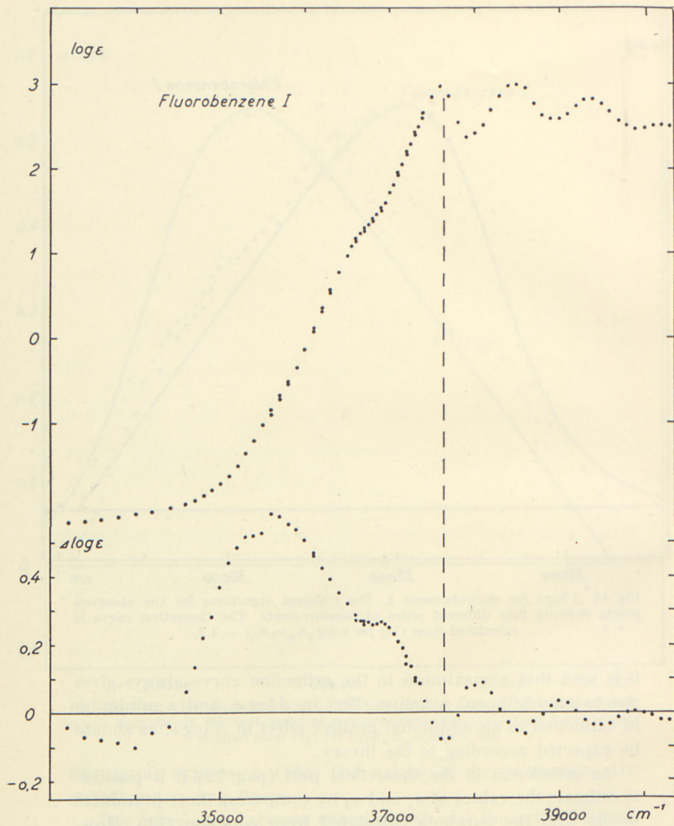
Fig. 15. \log \epsilon (25° C) and \Delta \log \epsilon for fluorobenzene.
