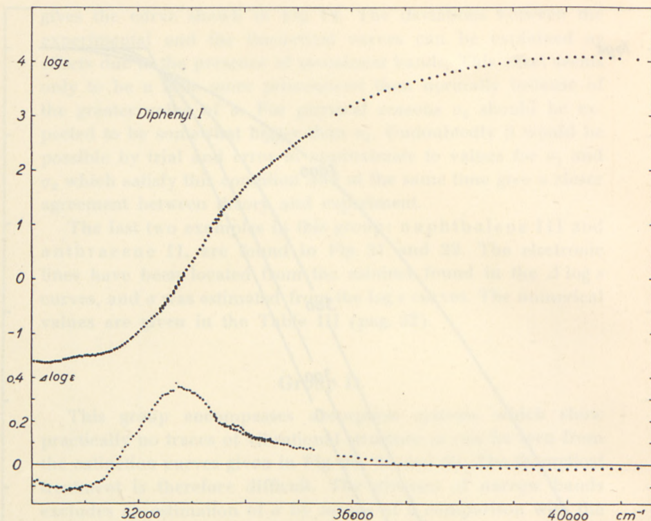
Fig. 24. \log \epsilon ( 25^{\circ}\text{C} ) and \Delta \log \epsilon for diphenyl.
