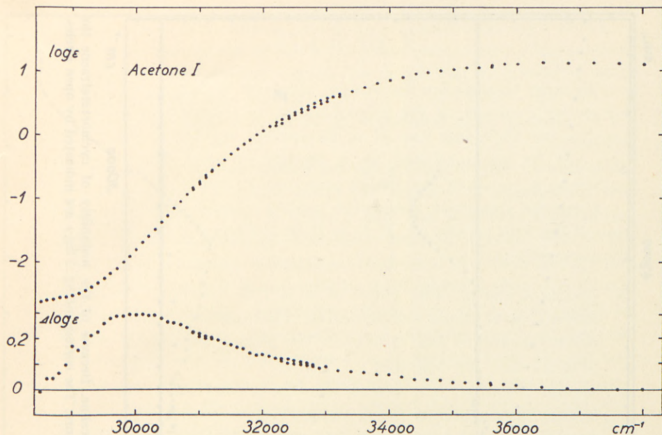
Fig. 25. \log \epsilon ( 25^\circ \text{C} ) and \Delta \log \epsilon for acetone.
