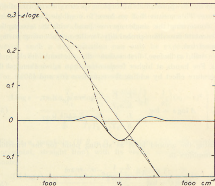
Fig. 9. The effect of a single, prominent band on \Delta \log \epsilon : — calculated from (56), and - - - from (58) for the usual temperatures.
