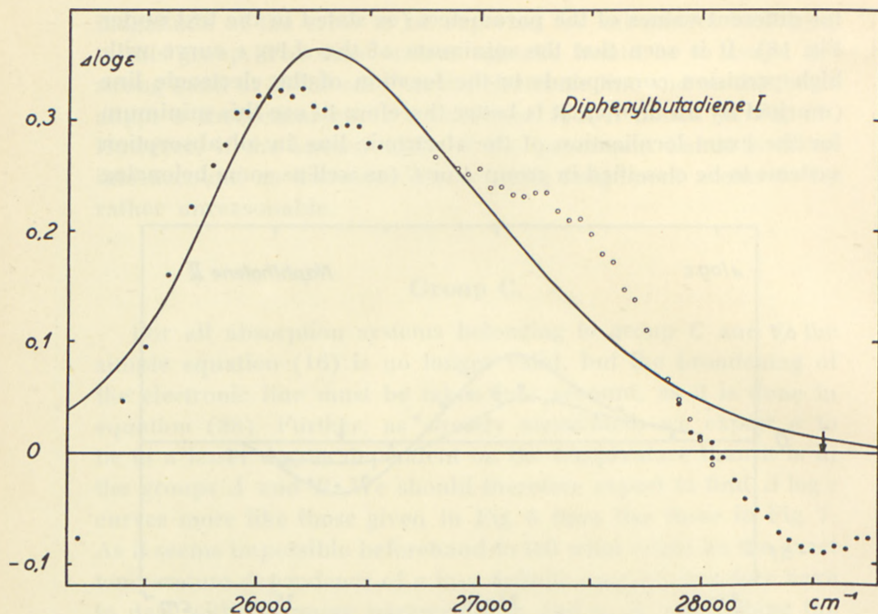
Fig. 19. \Delta \log \varepsilon for diphenylbutadiene I. The different signatures for the observed points indicate three series of measurements. The theoretical curve is calculated from (38) for \sigma_1 = \sigma_2 = 400 \text{ cm}^{-1} and \log (cK/c_0K_0) = 4.5 .
