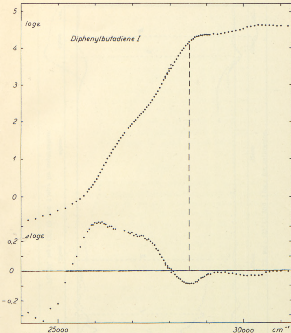
Fig. 20. \log \epsilon (25° C) and \Delta \log \epsilon for diphenylbutadiene.
