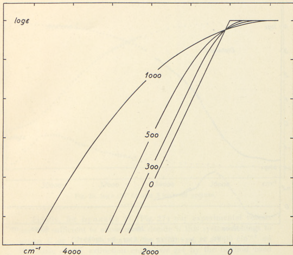
Fig. 23. Theoretical curves for \log \varepsilon = \log G calculated for T = 298^\circ K and for different values of \sigma as indicated. The ordinate is given in logarithmic units.
