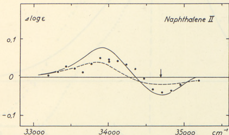
Fig. 18. \Delta \log \epsilon for naphthalene II. The theoretical curves are calculated from (61): — for \sigma_1 = \sigma_2 = 300 \text{ cm}^{-1} ; ---- for \sigma_1 = 300 \text{ cm}^{-1} and \sigma_2 = 325 \text{ cm}^{-1} .
