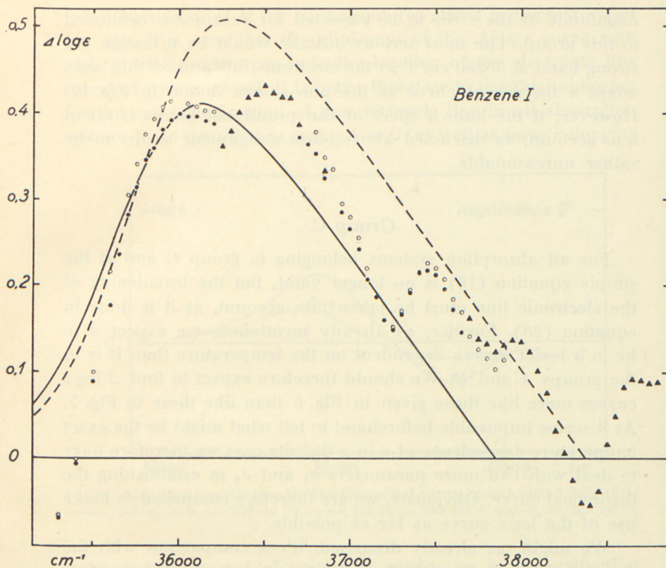
Fig. 17. \Delta \log \epsilon for benzene I. The different signatures for the observed points indicate six series of measurements. For theoretical curves see text.
