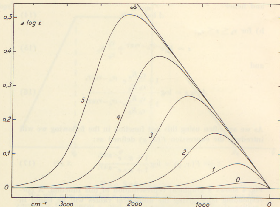
Fig. 4. \Delta \log \varepsilon = F(x, y) calculated for T_1 = 298^\circ \text{K} and T_2 = 343^\circ \text{K} . The numbers at the curves represent the parameter \log x = \log(c_a K_a / c_b K_b) .
